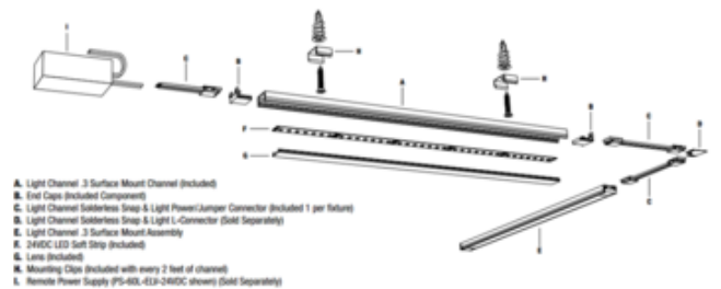
Included Components: Indoor Light Channel .3 Surface Mount system overview
