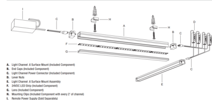
Components: Light Channel .6 Surface Mount system overview
