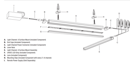
Components: Light Channel .6 Surface Mount system overview
