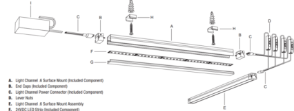
Components: Light Channel .6 Surface Mount system overview
