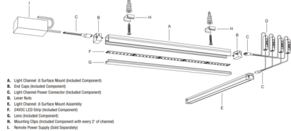
Components: Light Channel & Surface Mount system overview
