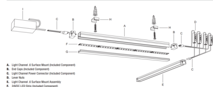
Components: Light Channel .6 Surface Mount system overview
