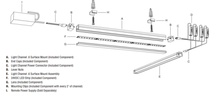
Components: Light Channel .6 Surface Mount system overview
