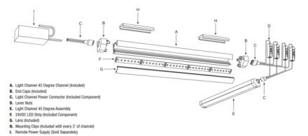
Components: Light Channel 45° system overview
