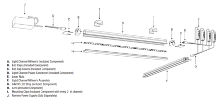
COMPONENTS: Light Channel 0.6" Millwork System Overview
