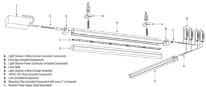
COMPONENTS: Light Channel .6 Micro Grazer system overview
