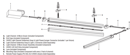
Included Components: Light Channel .6 Micro Grazer system overview
