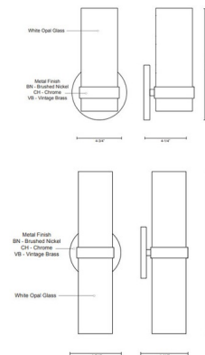
Shown in brushed nickel / white opal
