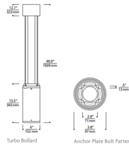
Turbo Bollard Anchor Plate Bolt Pattern
