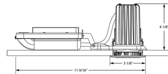
TRIM/LED ASSEMBLY
