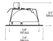
RETROFIT HOUSING
