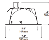
RETROFIT HOUSING
