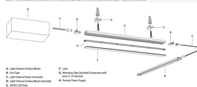
LIGHT CHANNEL SURFACE MOUNT SYSTEM OVERVIEW: TRADITIONAL DIMMING, 0-10, DMX AND DALI
