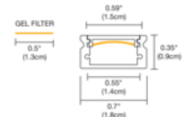
LCS.3 Light Channel Diffused Lens with Gel Color Filter (provided by customer)
