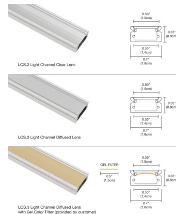
Shown in satin aluminum / diffused lens
