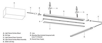
LIGHT CHANNEL SURFACE MOUNT SYSTEM OVERVIEW: TRADITIONAL DIMMING, 0-10, DMX AND DALI
