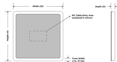
DIMENSIONAL DRAWING (Not to scale. Frost and border widths may vary depending on mirror size)
