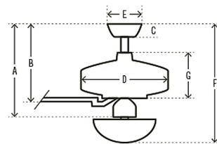
42" and 52" Fans
