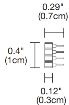
Female Connector
