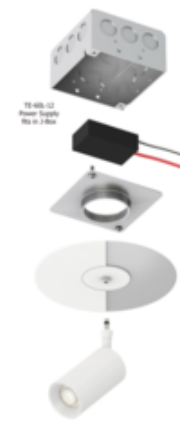
WPM-4113 Vanishing Point 2" Flush Canopy to dry wall plaster in and paint, with 6" power supply in 2.5A
