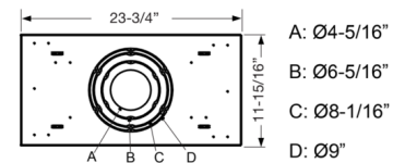
T-Grid
