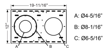
Stud/Joist
