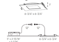
SPN6SQ-CC-3T - 6" Square Panel Light With Interchangeable Trims
