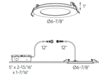
SPN6-CC-3T - 6" Round Panel Light With Interchangeable Trims
