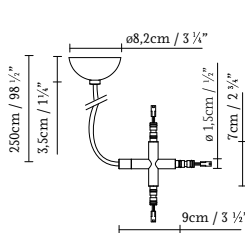
KUPETZ XH POWER SUPPLY
