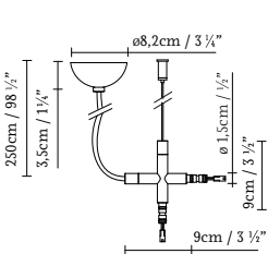
KUPETZ XS POWER SUPPLY
