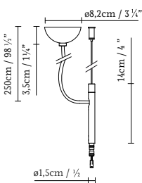
KUPETZ S POWER SUPPLY
