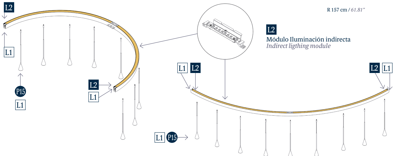
Luminaria Skybell Cono de iluminancia (indirecta) Skybell light illuminance cone (indirect)
